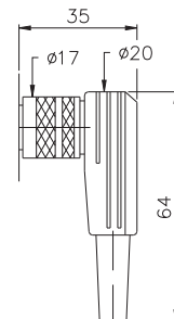
CON013 - IP40 Prot. (DIN43322 - 5 pole Female connector)
