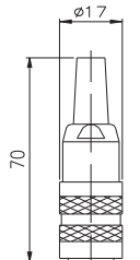
CON006 - IP65 Prot. (DIN43650 - 4 pole Female connector)
